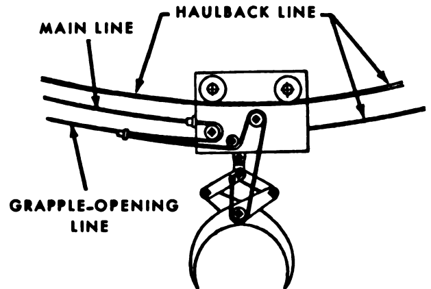
Figure 7-24. Logging grapple and carriage.
